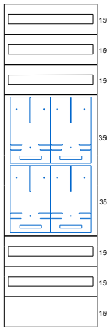
RWX 4L-S1600 550x1600x250
