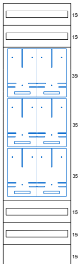
RWX 6L-S1800 550x1800x250
