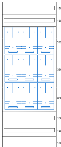
RWX 9L-S1800 750x1800x250
