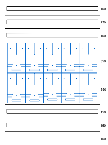
RWX 10L-S1600 1150x1600x250
