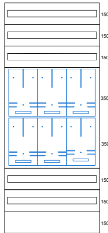
RWX 6L-S1600 750x1600x250
