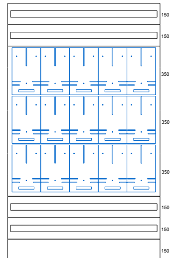
RWX 15L-S1800 1150x1800x250
